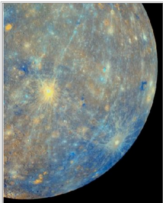
This is a mosaic of images collected by MESSENGER as it departed Mercury on October 6, 2008. The Wide Angle Camera on MESSENGER imaged the surface through 11 color filters ranging in wavelength from 430 to 1020 nm. A principal component analysis of the 11 sets of images helps to highlight subtle color differences. The second principal component, first principal component, and a ratio of the 430 nm to 1020 nm wavelengths are combined here in a red-green-blue composite. Impact craters that formed relatively recently, such as Kuiper (62 km in diameter, yellow crater near center), have contrasting ejecta and rays because they excavated fresh material. As it sits on the surface, this fresh crater material will gradually alter its color until it matches the background material. Other impact craters, such as those with ejecta that appear blue in this color scheme, have color contrasts because they excavated compositionally distinct material from below the surface. Lermontov crater (152 km in diameter), near the top left, appears orange and is thought to contain pyroclastic deposits resulting from explosive volcanic activity in the past. - Credit: NASA/Johns Hopkins University Applied Physics Laboratory/Arizona State University/Carnegie Institute of Washington
