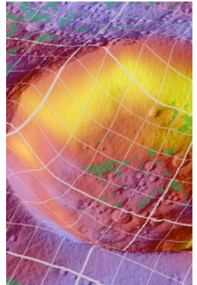
This is an artist's rendition of LRO's temperature map of a crater. Credit: NASA
