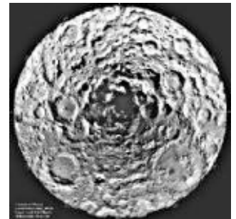
Lunar Clementine mission shows the South Pole of the Moon. The permanently shadowed region center showed earlier evidence of meteor cratering and ice never exposed to direct sunlight, but Arecibo radar reveals dust. Credit: NASA/DOD Clementine
